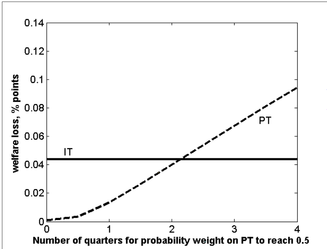
Figure 3: Benchmark results: Welfare losses of various monetary policy regimes minus welfare loss of PT under perfect credibility. Solid line is for IT, dashed curve is for PT with various degrees of imperfect credibility under Scenario 1 (various speeds of gradual adjustment in credibility).
