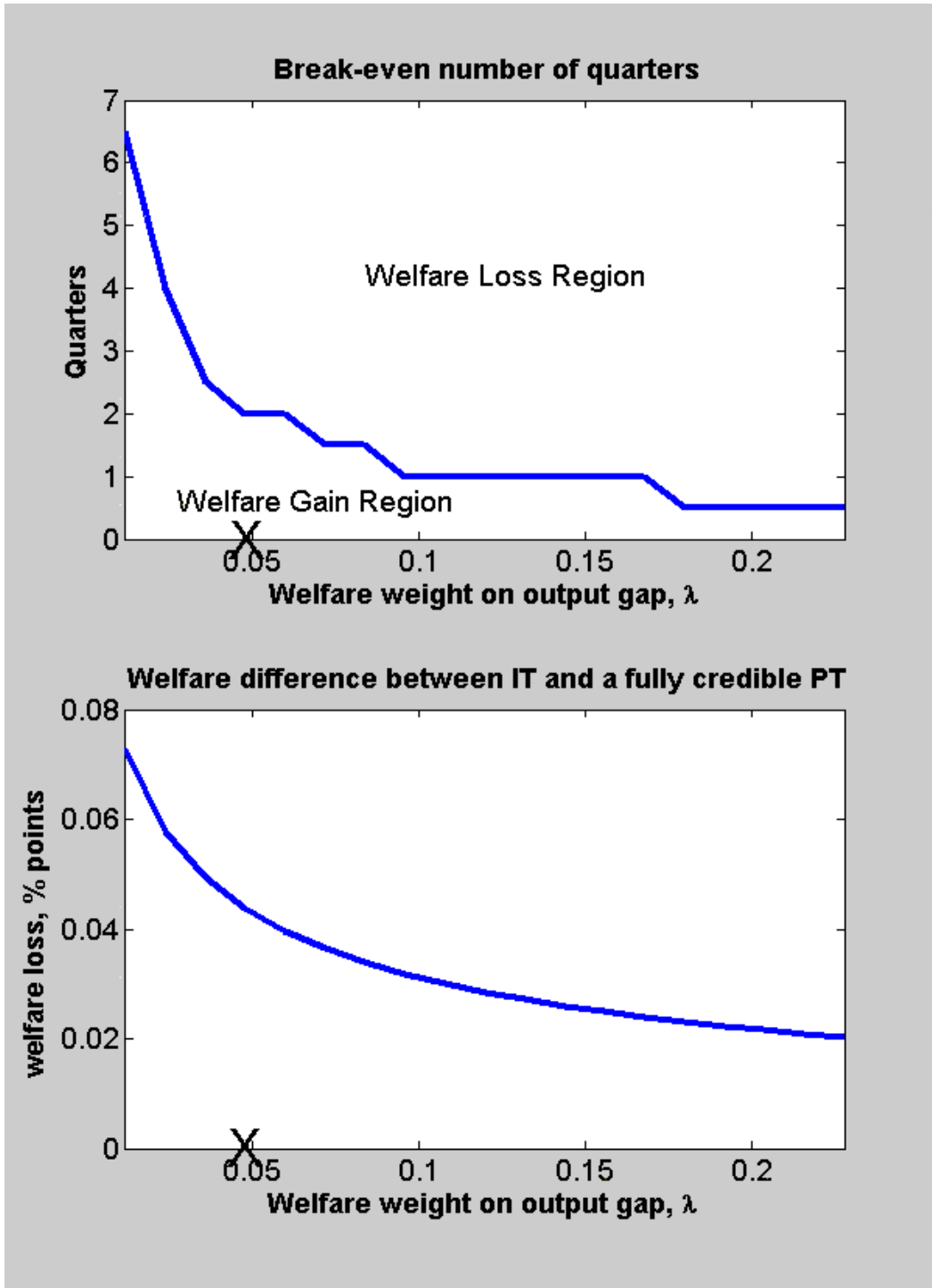
Figure 6: Sensitivity Analysis: The top chart shows Net Welfare Gain and Net Welfare Loss regions for range of values of the welfare weight on output gap. The curve shows break-even number of quarters for the "half-time" of gradual adjustment (Scenario 1). X signifies the benchmark value of the welfare weight on output gap. The bottom part shows the welfare difference between IT and a fully credible PT.
