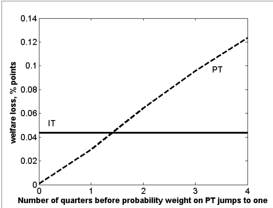
Figure 4: Benchmark results: Welfare losses of various monetary policy regimes minus welfare loss of PT under perfect credibility. Solid line is for IT, dashed curve is for PT with various degrees of imperfect credibility under Scenario 2 (various speeds of jump adjustment in credibility, T).
