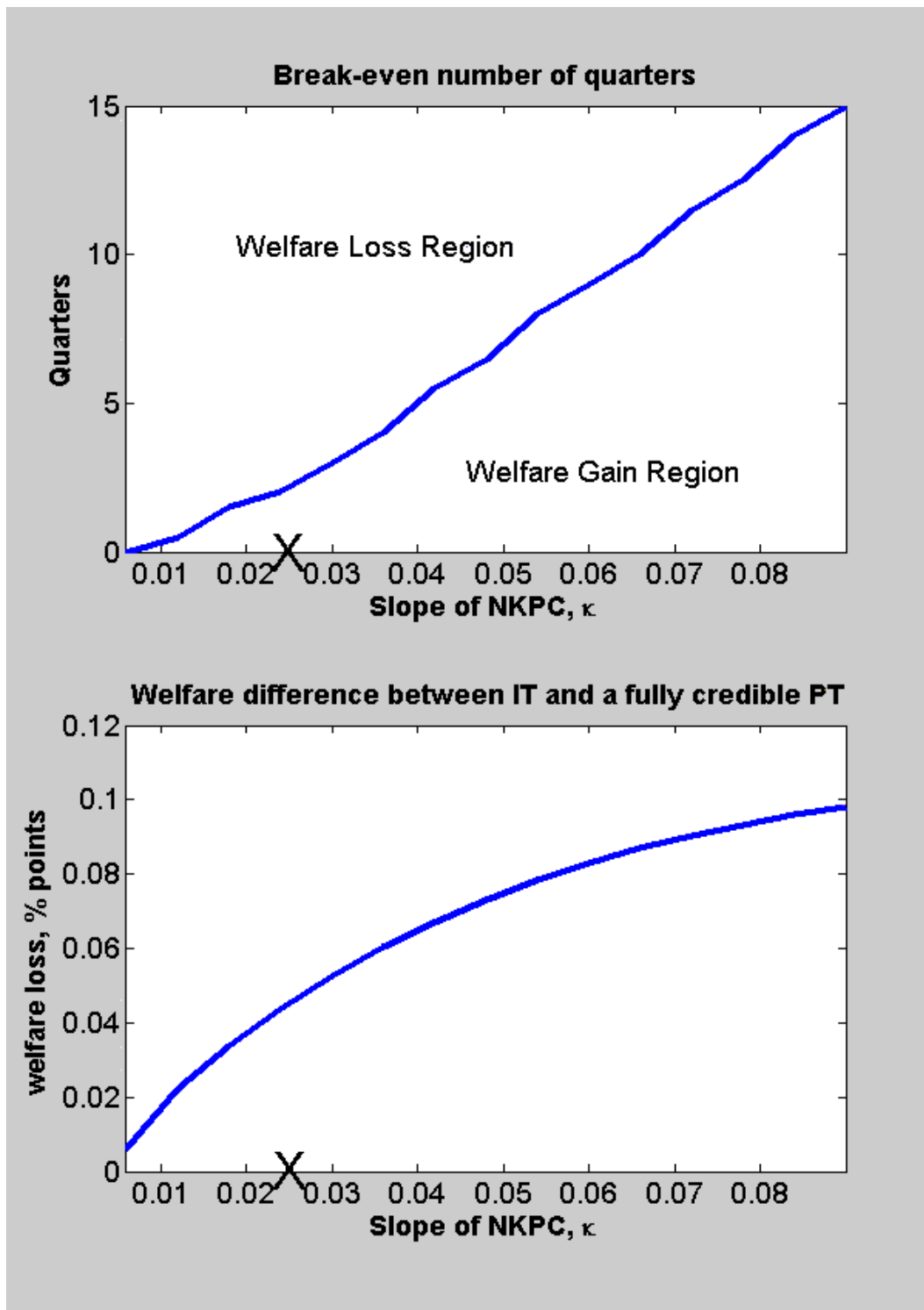
Figure 7: Sensitivity Analysis: The top chart shows Net Welfare Gain and Net Welfare Loss regions for range of values of the slope of the Phillips curve. The curve shows break-even number of quarters for the “half-time” of gradual adjustment (Scenario 1). X signifies the benchmark value of the slope. The bottom part shows the welfare difference between IT and a fully credible PT.
