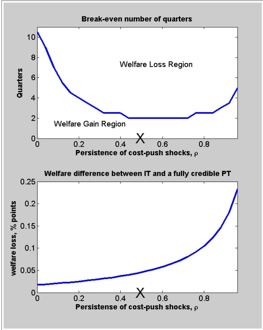
Figure 5: Sensitivity Analysis: The top chart shows Net Welfare Gain and Net Welfare Loss regions for range of values of the persistence of cost-push shocks. The curve shows break-even number of quarters for the "half-time" of gradual adjustment (Scenario 1). X signifies the benchmark value of the persistence parameter. The bottom part shows the welfare difference between IT and a fully credible PT.
